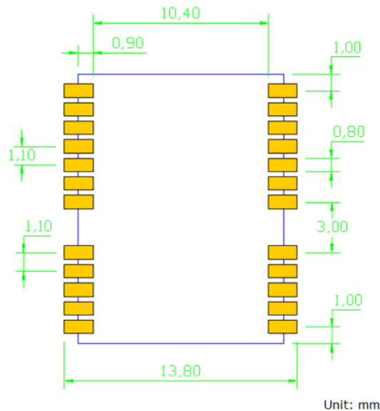
Figure 6: Footprint of Recommendation (Unit: mm)
