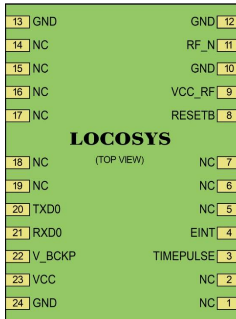
Figure 4: Pin Assignment
