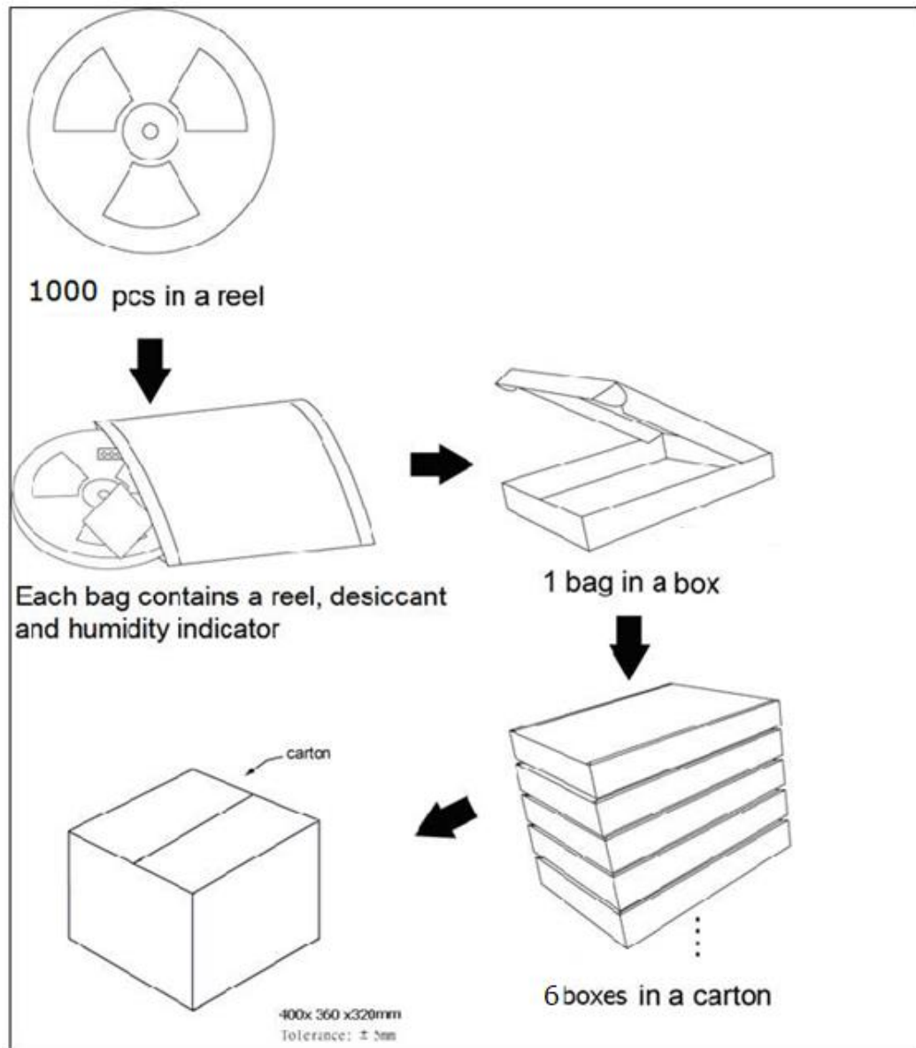
Figure 8: Packing method
