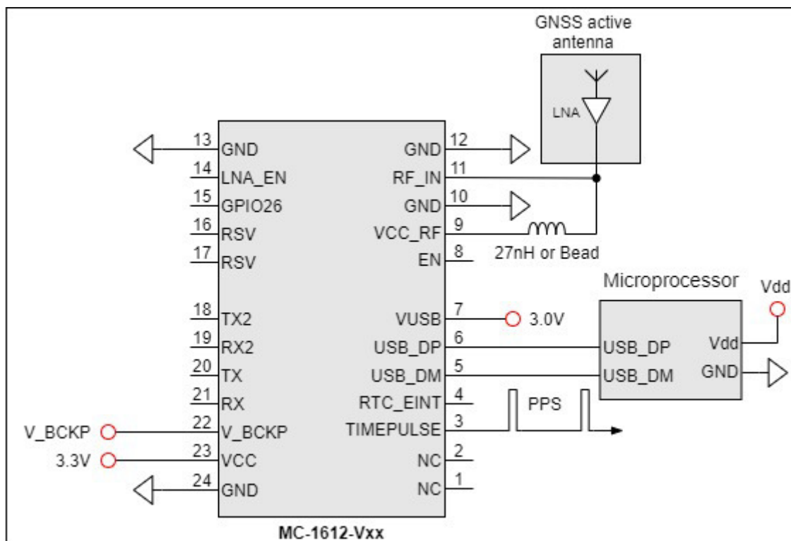
Fig 3-3 Typical application circuit that uses USB interface.
