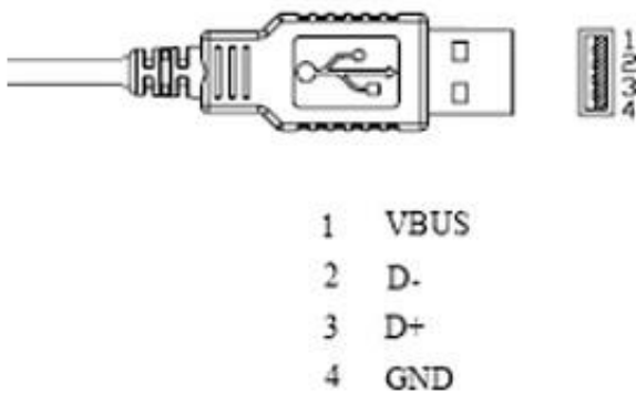
Figure 2: USB Pin Assignment
