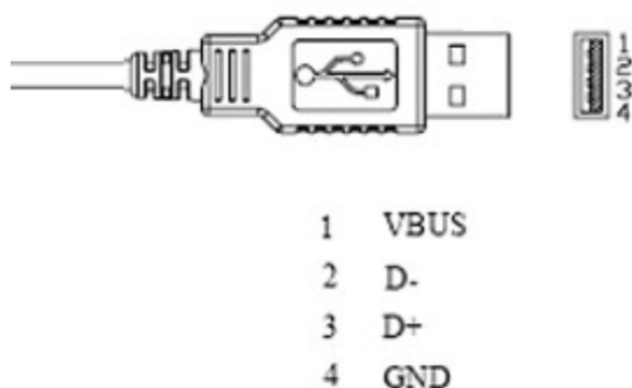
Figure 2: USB Pin Assignment
