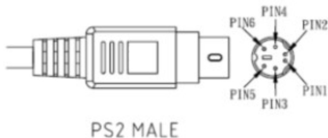
Figure 3: PS2 Pin Assignment
