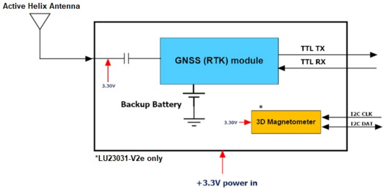
Fig 3-1 System block diagram of LU23031-V2 , LU23031-V2e
