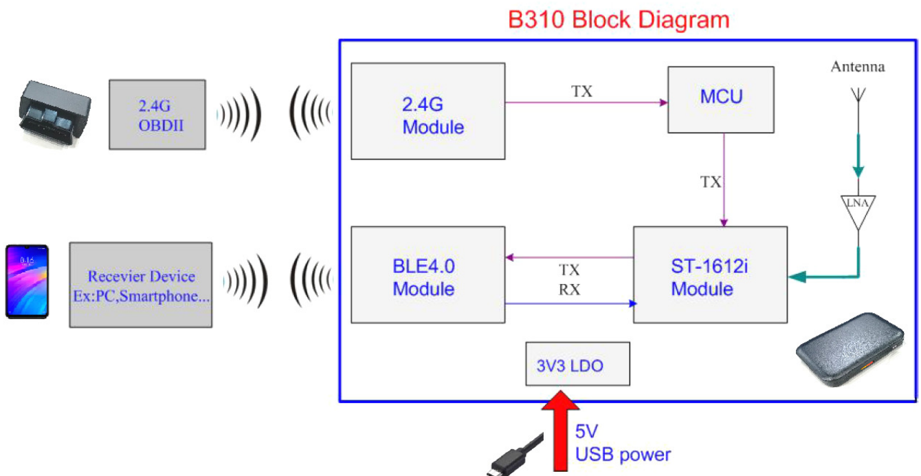
Fig 4-1 System block diagram.
