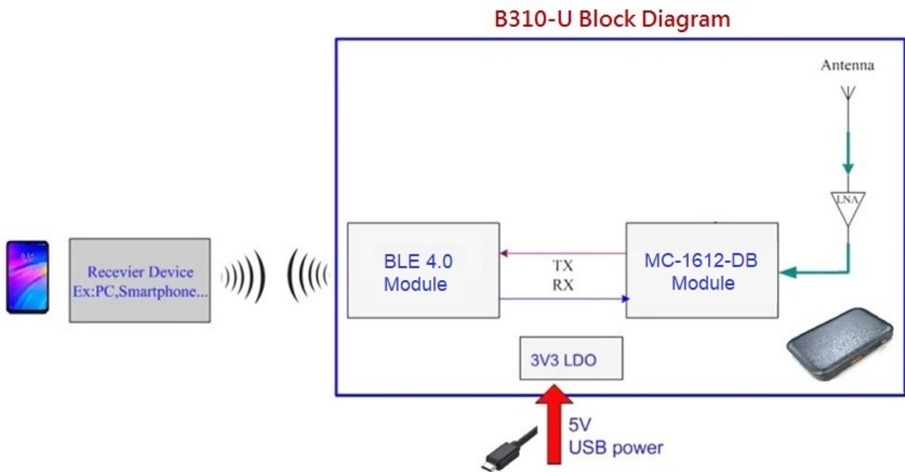
Fig 4-1 System block diagram
