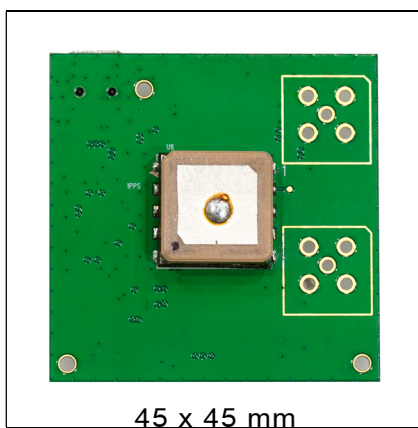
Fig 4-1 Evaluation board of LS2003C
