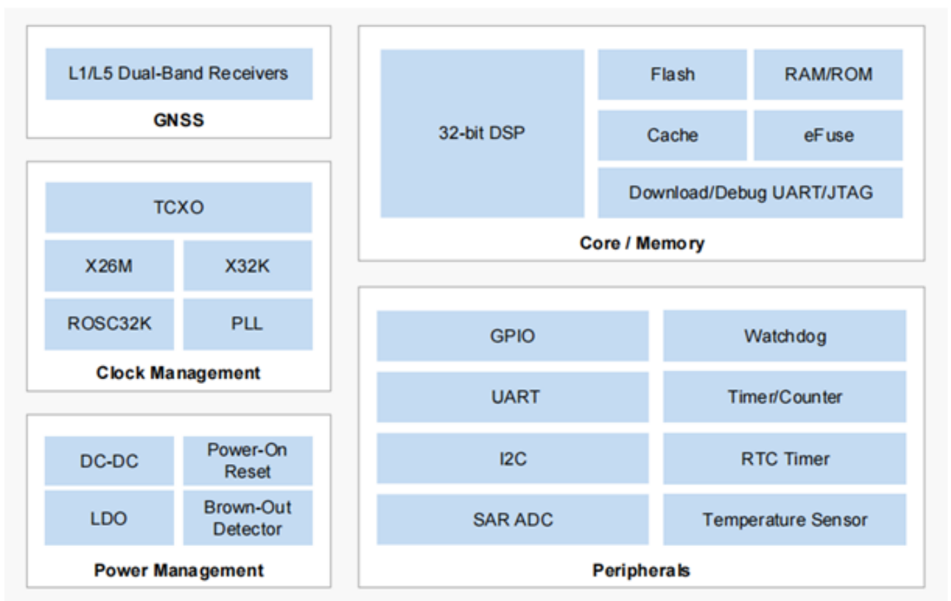
Figure 1: Block Diagram
