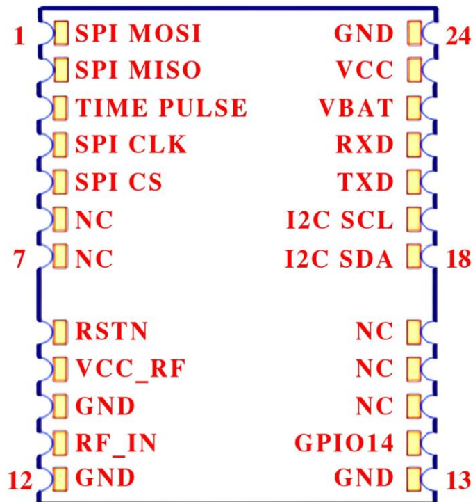
Figure 2: Pin Assignment
